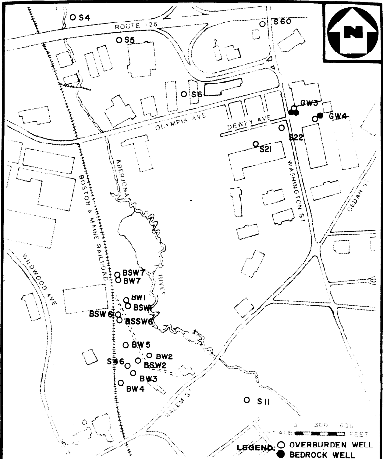
SAMPLING LOCATIONS (INITIAL ROUND JULY 1984) WELLS G AND H WOBURN, MA
