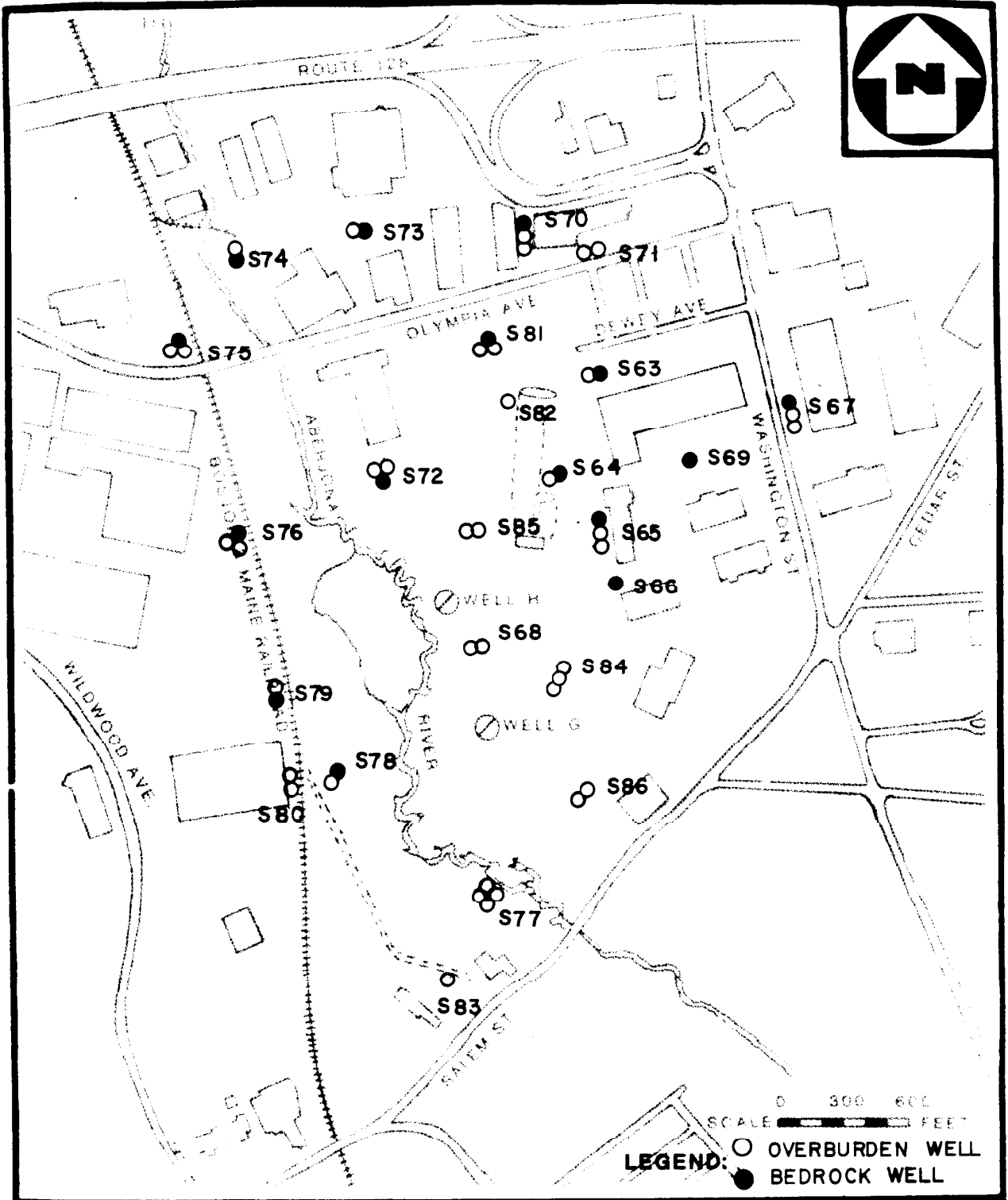
NUS/ FIT MONITORING WELL LOCATIONS WELLS G AND H WOBURN, MA
