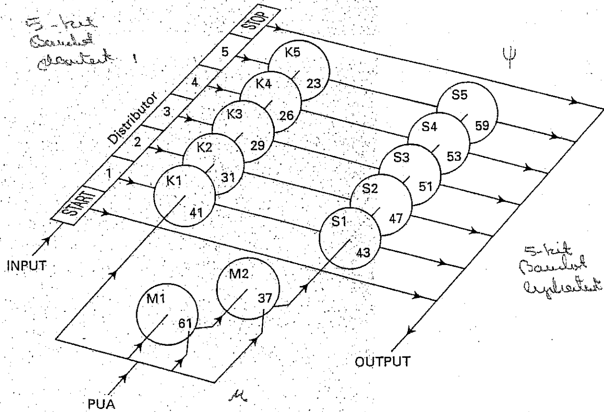
Motor wheel FIG. 20.1. The Tunny machine
