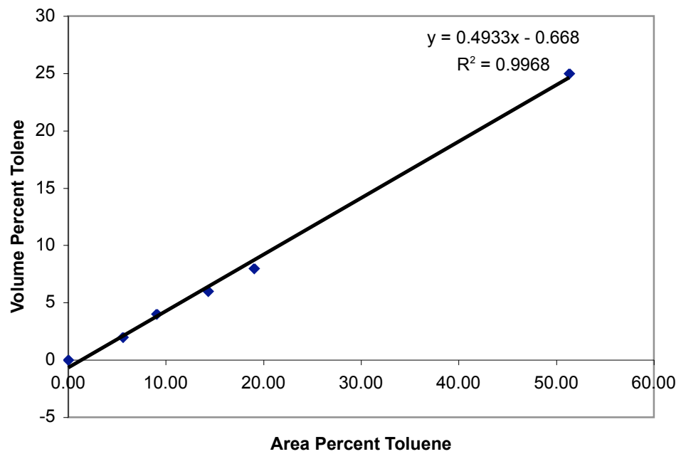
Volume - Area Relationship for Toluene in Acetone
